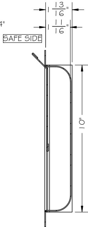
THREAT SIDE SECTION A-A
